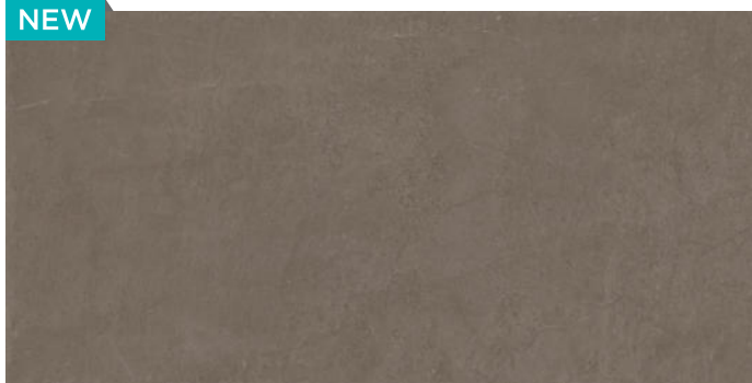
Panora Bruno
