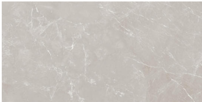
Tunisia Polished
